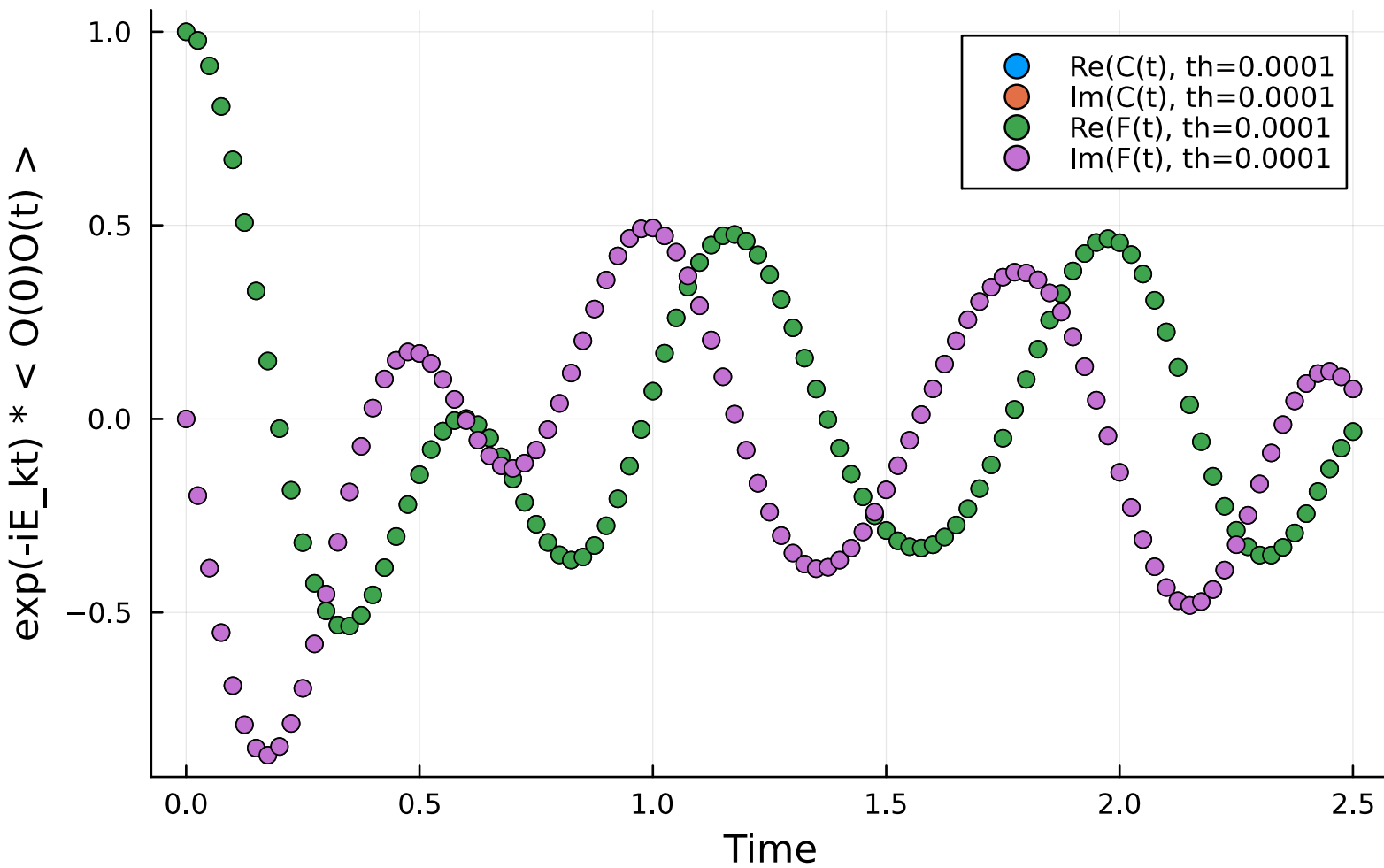
Signal Comparison N=6, J=1.0, Jz=2.0, dt=0.025
