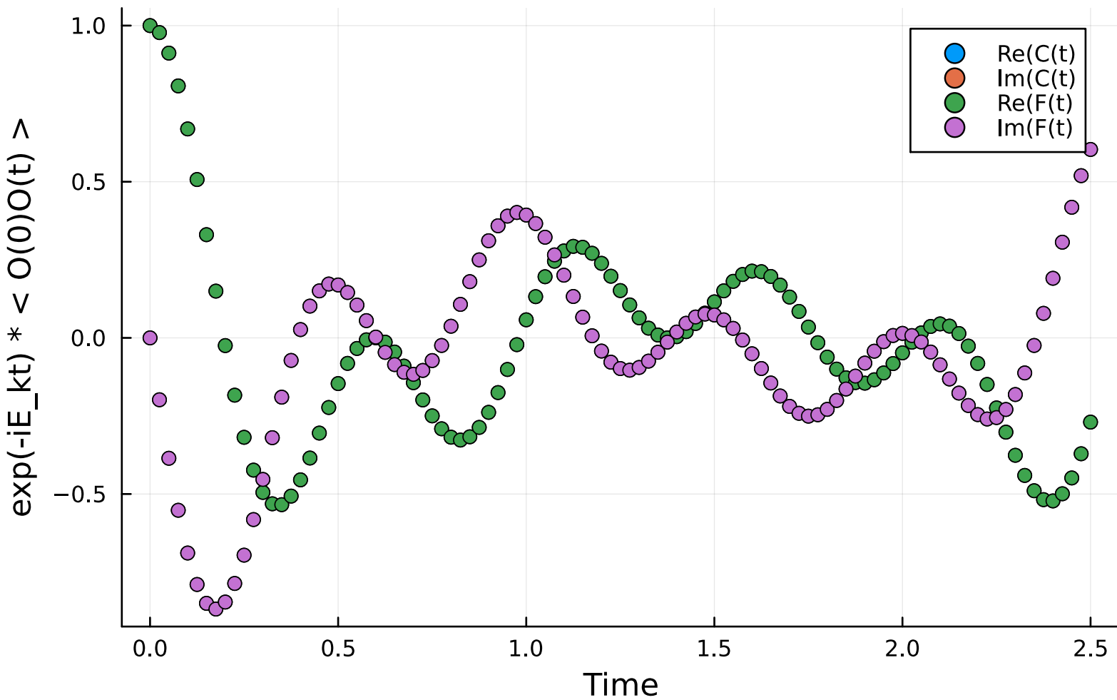
Signal Comparison N=10, J=1.0, g=0.0, dt=0.025
