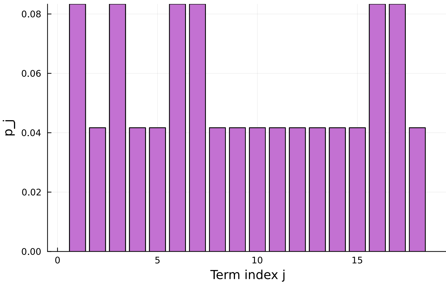
qDRIFT sampling distribution ( \lambda = 24 )
