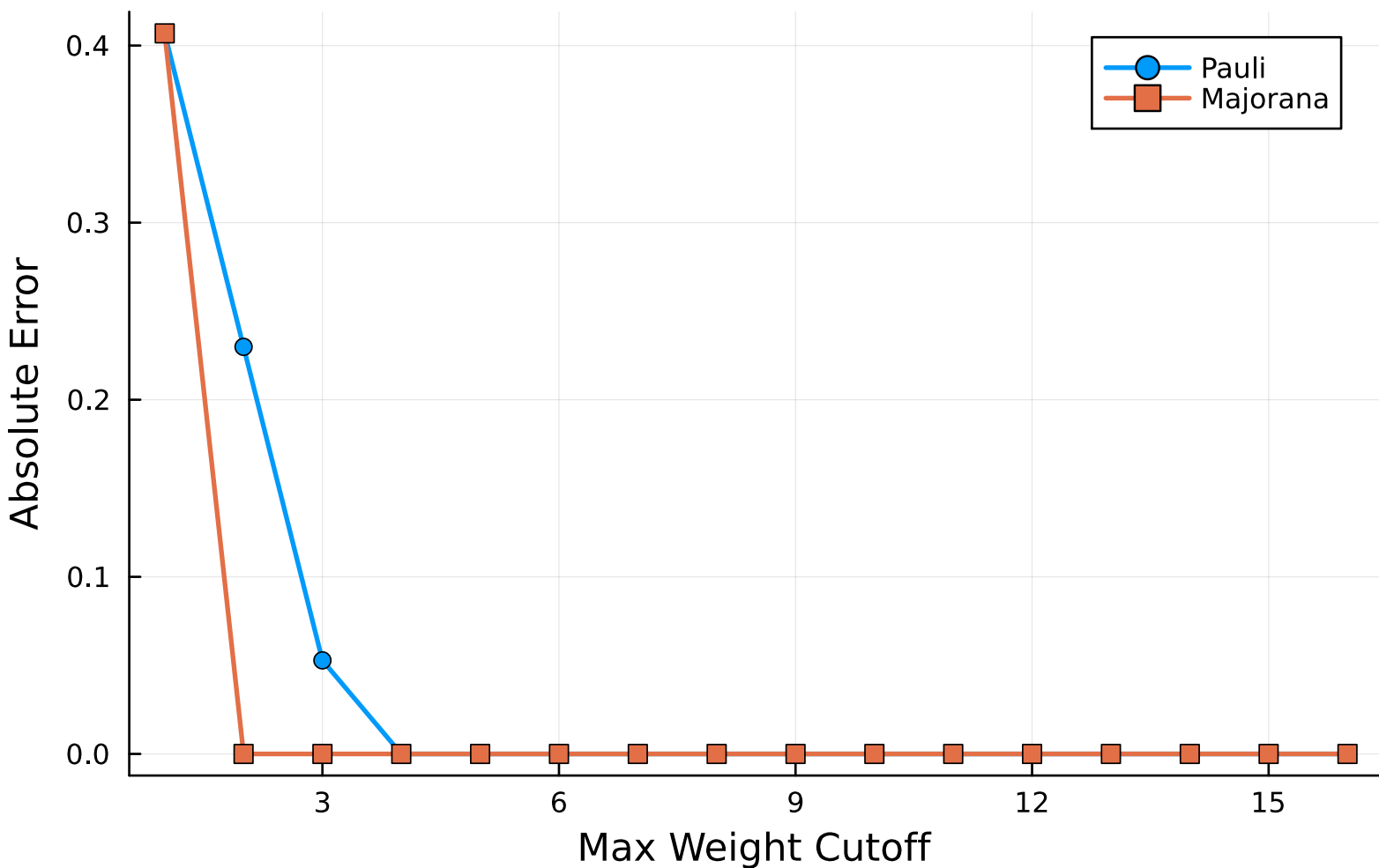
Error vs Max Weight (Lx=2, Ly=2, U=4.0)
