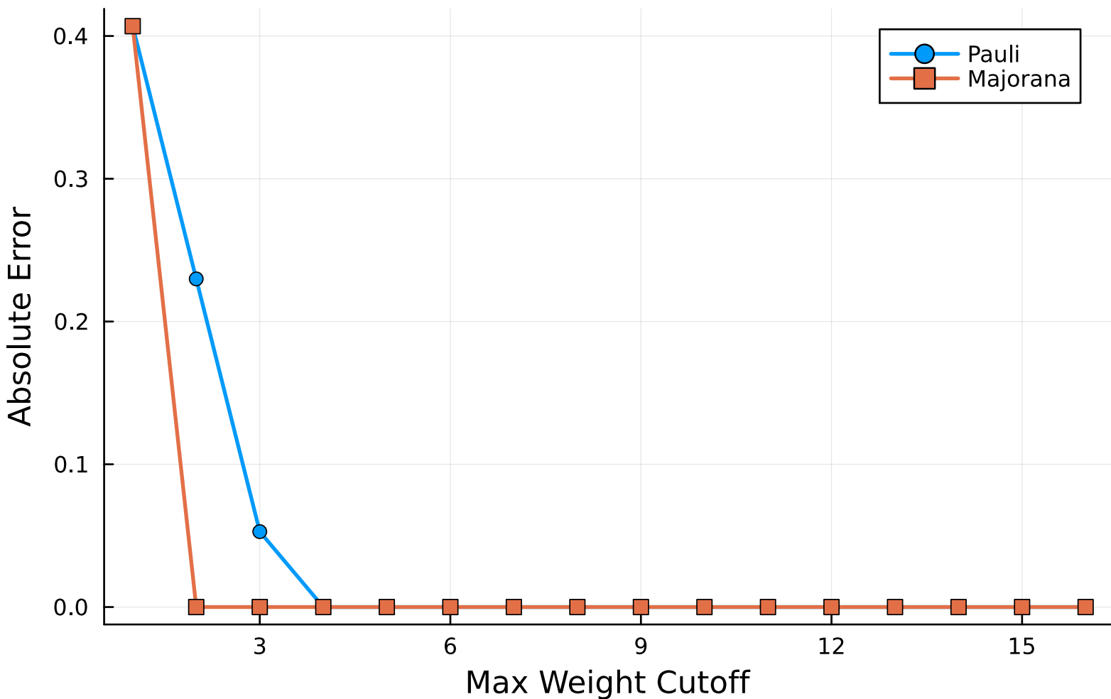
Error vs Max Weight (Lx=2, Ly=2, U=8.0)
