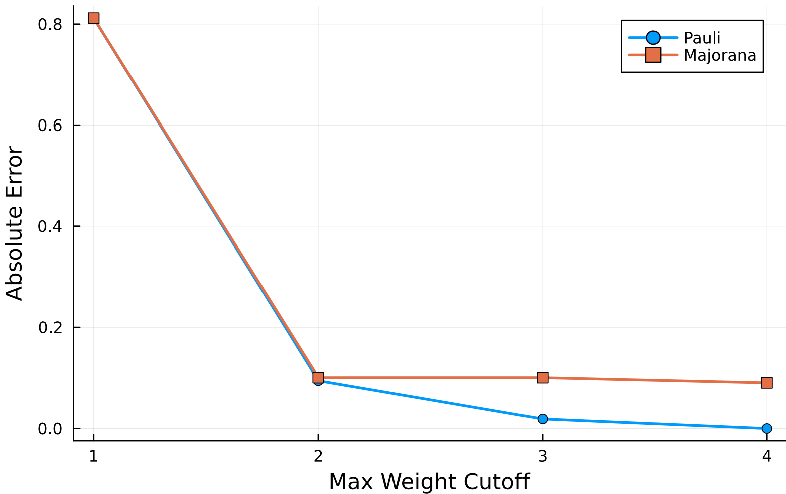
Error vs Max Weight (N=4, k=6)
