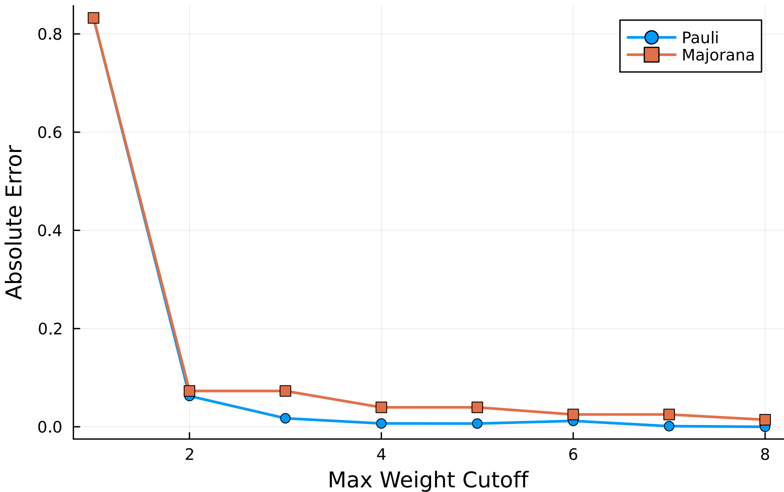
Error vs Max Weight (N=8, k=6)
