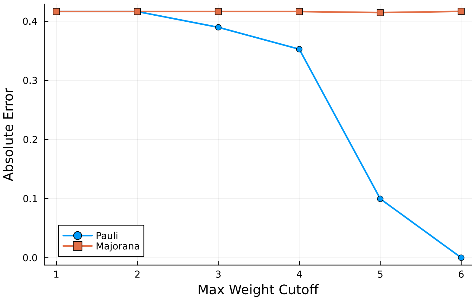
Error vs Max Weight (N=6, k=10)
