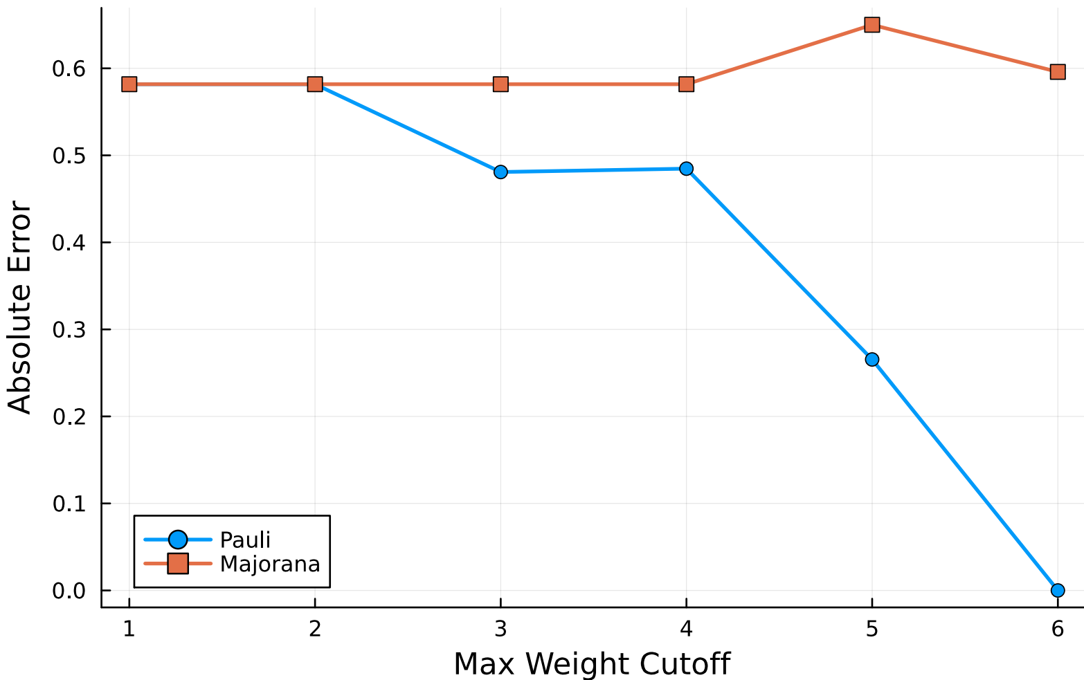
Error vs Max Weight (N=6, k=6)
