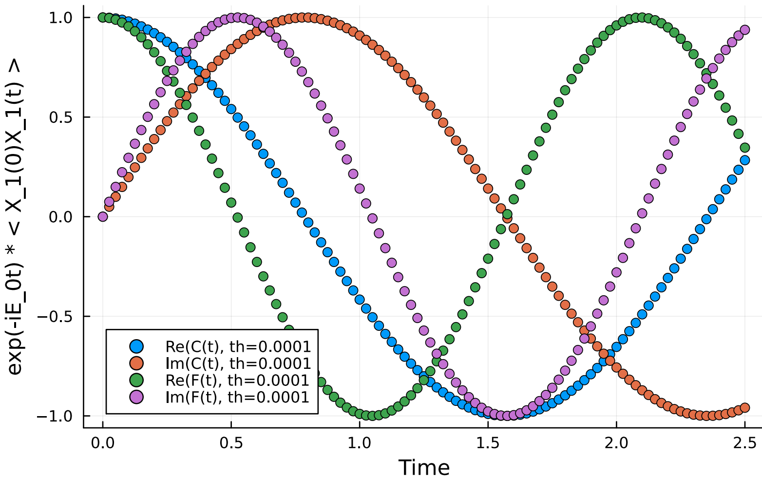
Signal Comparison N=4, J=1.0, g=0.0, dt=0.025
