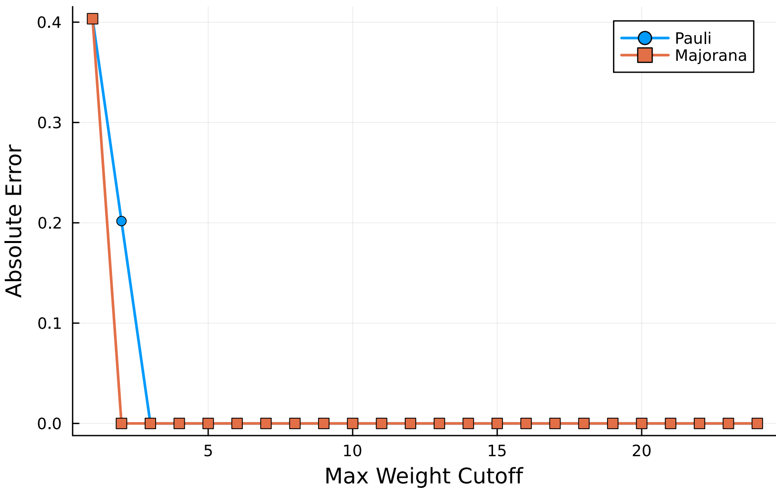
Error vs Max Weight ( L_x=2 , L_y=3 , U=0.0 )
