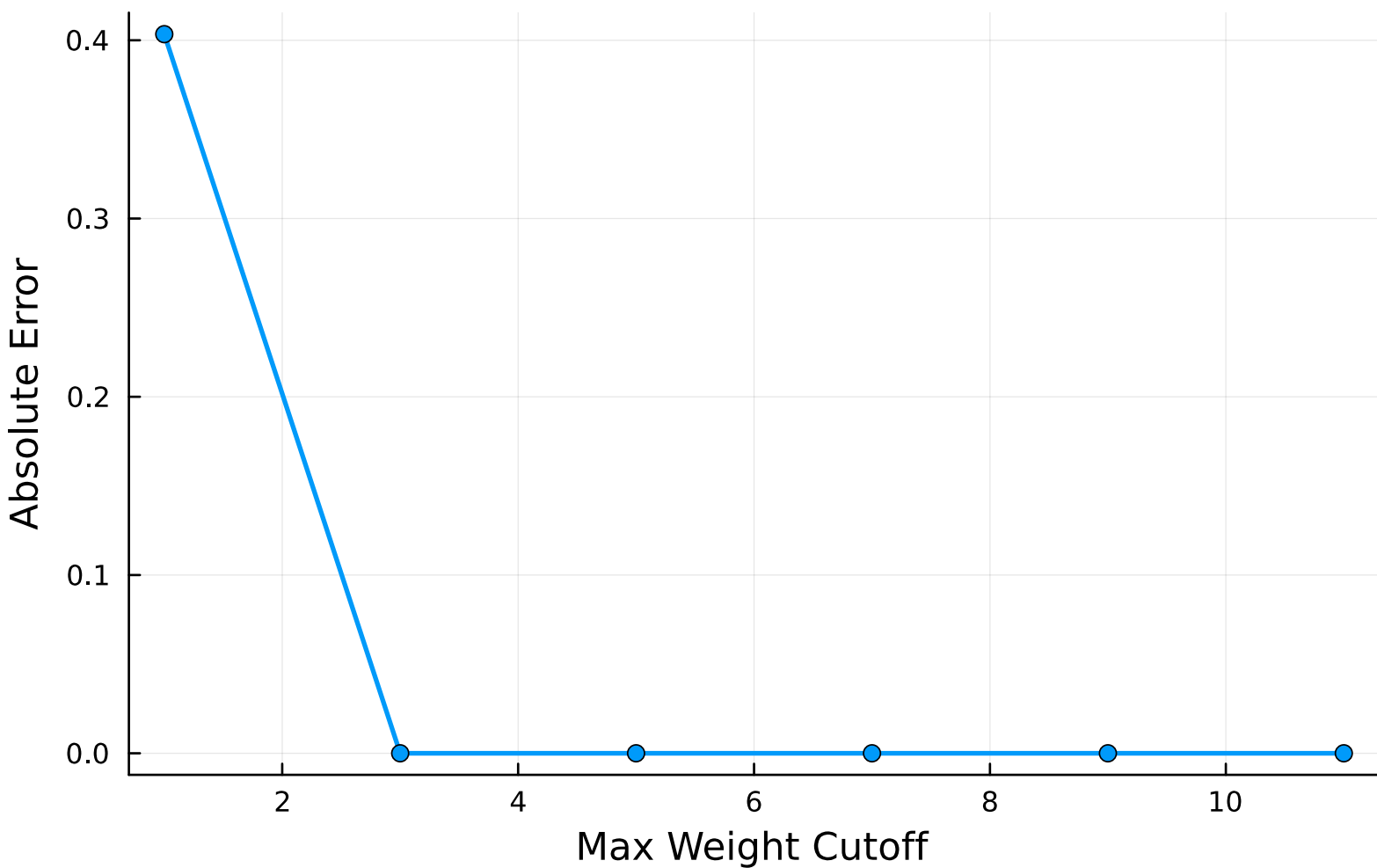
Error vs Max Weight Cutoff (Hubbard, U=1.0 , t=-1.0 )
