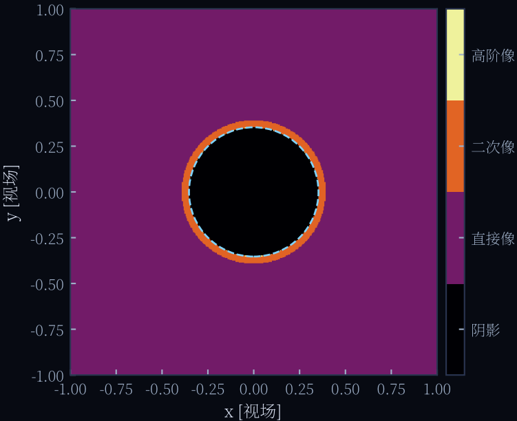
视线与赤道面交会的像阶 ( r_0 = 26M )
