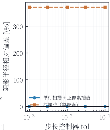
(b) 阴影半径的收敛
