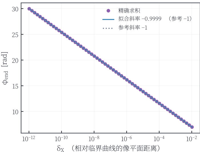
(c) 每十倍 \delta_X 只多绕 \ln 10 (= 2.303 \text{ rad})
