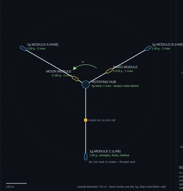
VIEW A — PLAN, LOOKING ALONG THE SPIN AXIS ( \omega OUT OF PAGE, COUNTER-CLOCKWISE)
