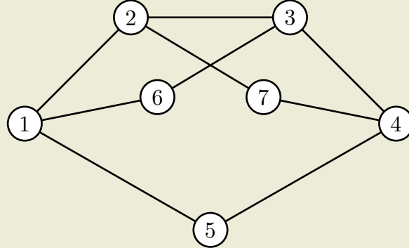
Figure 1: Graph for the k -coloring problem
