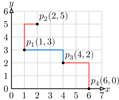
Figure 5: The Minimum Spanning Tree.
