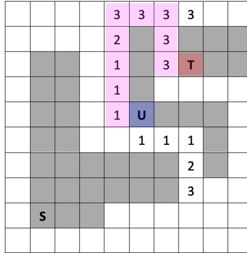
Figure 9: Finding the shortest path between U to T by Hadlock's approach. The number labeled in each grid is the detour number.
