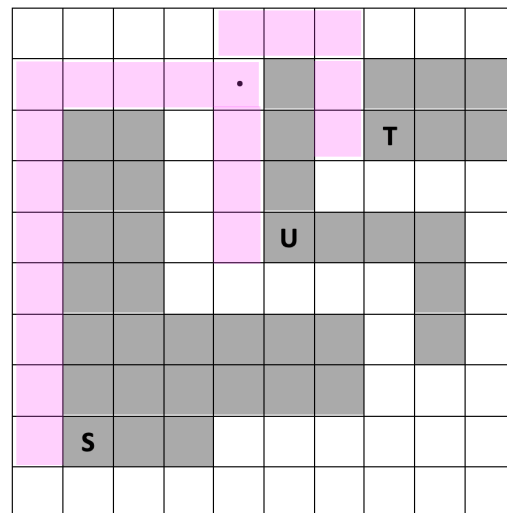
Figure 11: The Steiner tree connecting S, U, and T.
