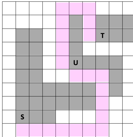
Figure 10: The minimum spanning tree connecting S, U, and T. The total length of the tree is 24.
