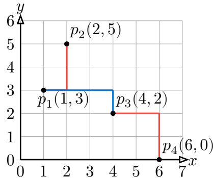
Figure 6: The Minimum Steiner Tree.
