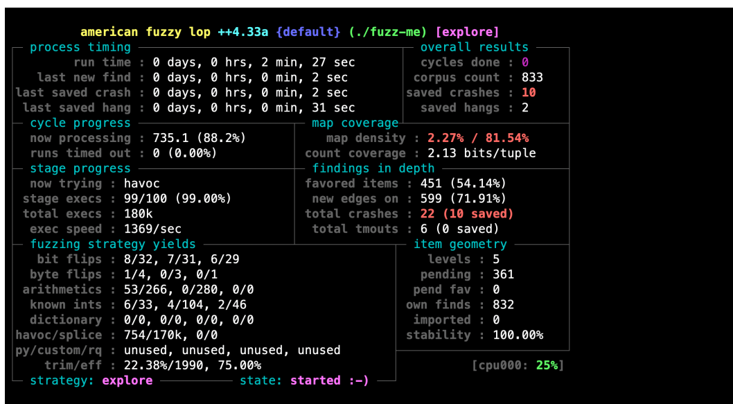
Figure 6: AFL++ fuzzing 介面
