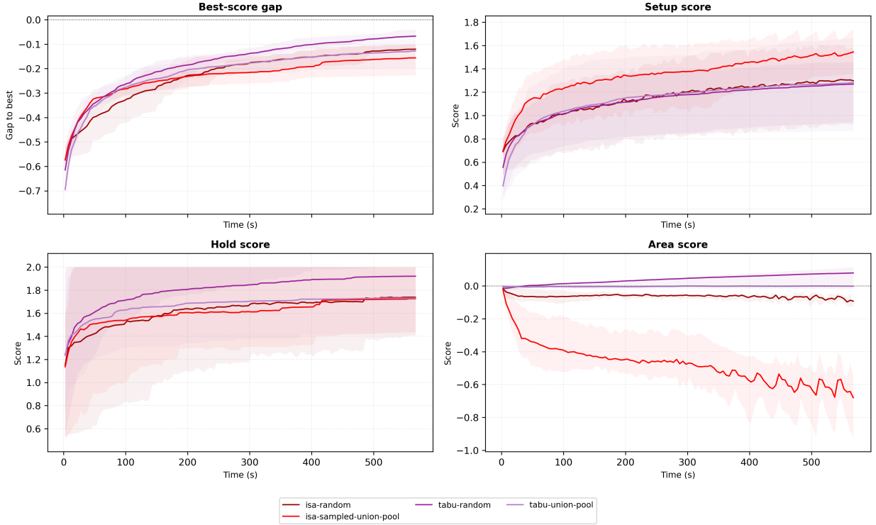
Figure 4: Direct comparison between ISA and tabu variants. The figure compares random and union-based variants of ISA and tabu search using the same four trajectory components.
