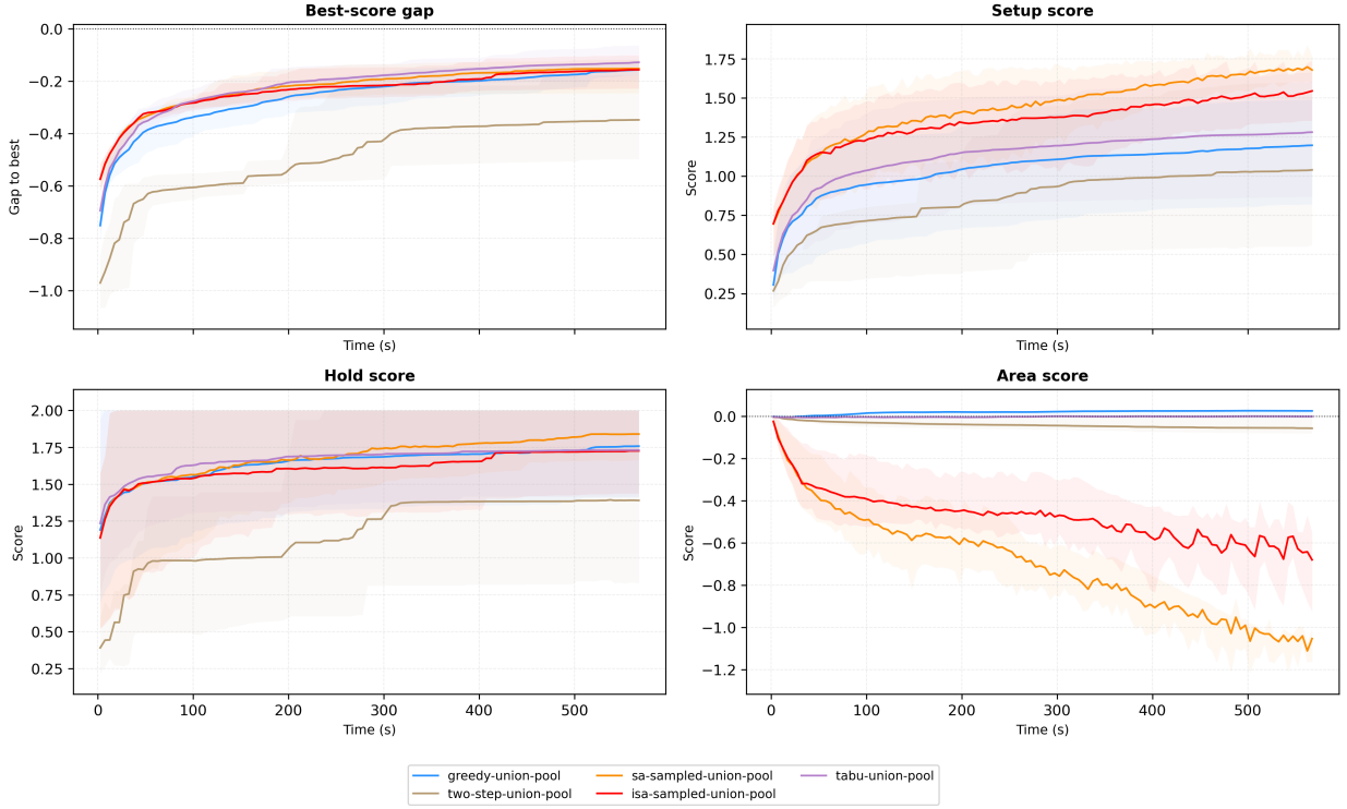
Figure 3: Acceptance-policy comparison under union-based candidate policies. Greedy, two-step, and tabu use the union pool, while SA and ISA use sampled union-pool proposals.
