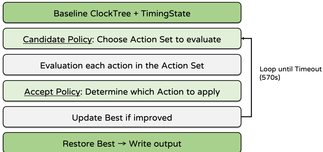
Figure 1: Overall local-search framework of our solver. Each iteration consists of candidate generation, candidate evaluation, move acceptance, and best-state update. The best-seen clock tree is restored and written to the output after the time budget is reached.
