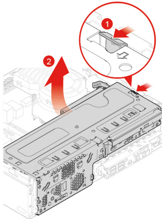
Figure 37. Pivoting the drive bay assembly upward
