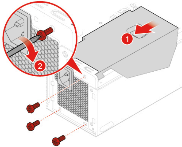
Figure 109. Installing the power supply assembly
