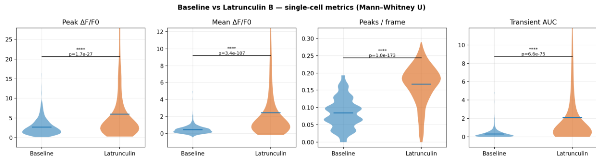
Figure 9. Single-cell metric distributions, baseline vs Latrunculin B, pooled across two trials (descriptive; the pooled per-cell p-values annotated here are pseudoreplicated — see §3.1). The length-normalized transient rate and per-frame area are the sound metrics.
