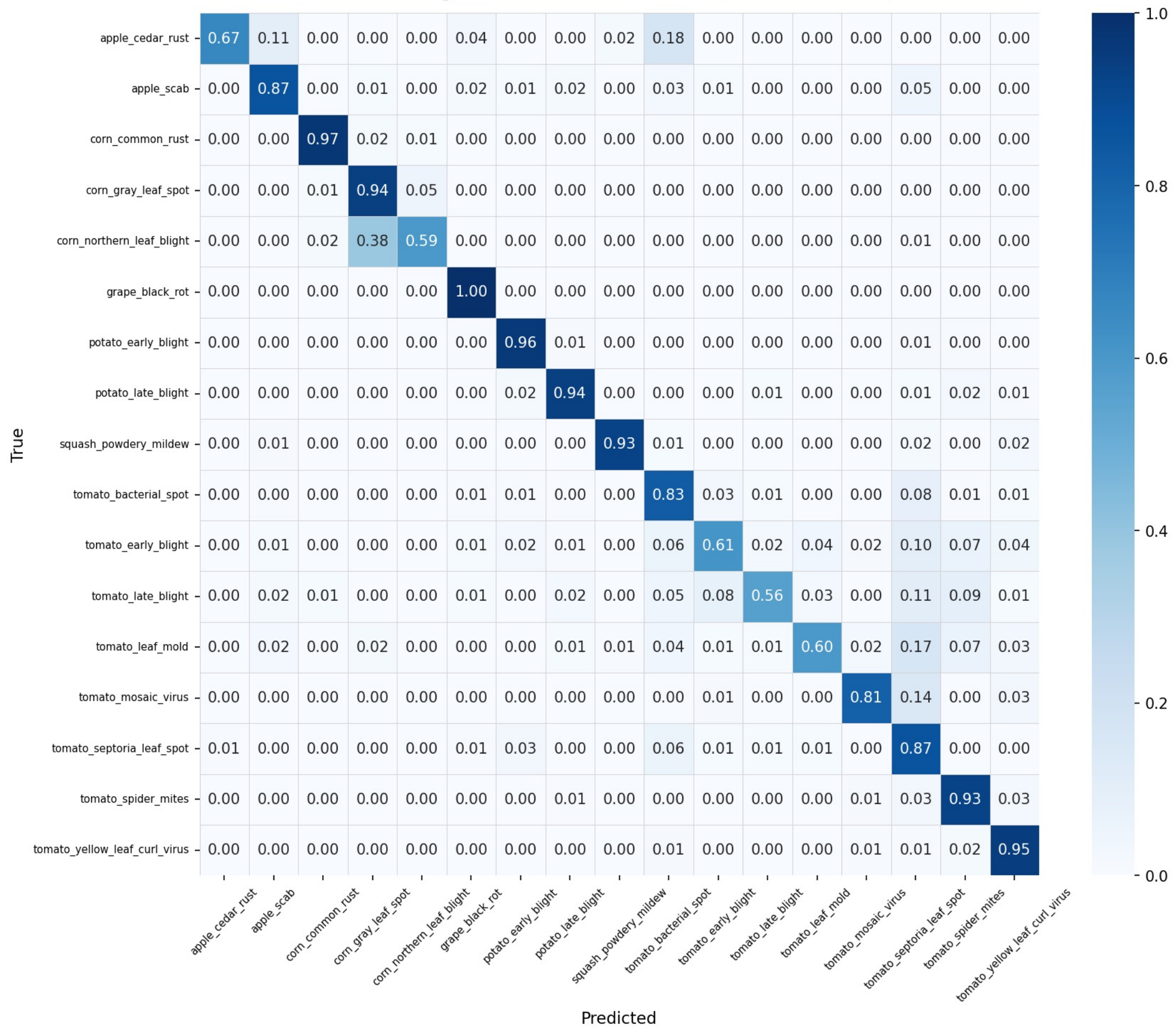
PlantVillage Val — Confusion Matrix (row-normalised)
