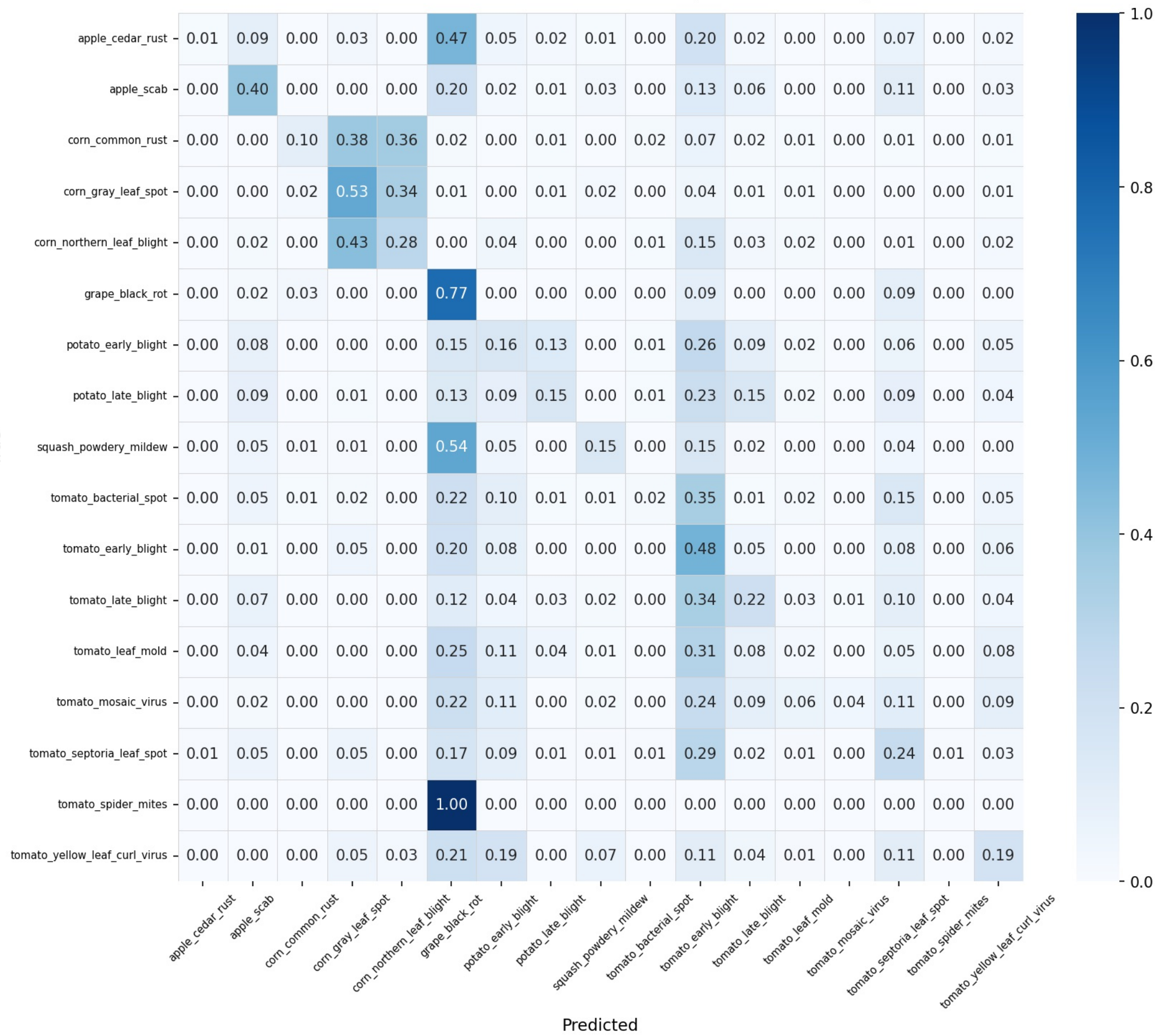
PlantDoc Eval — Confusion Matrix (row-normalised)
