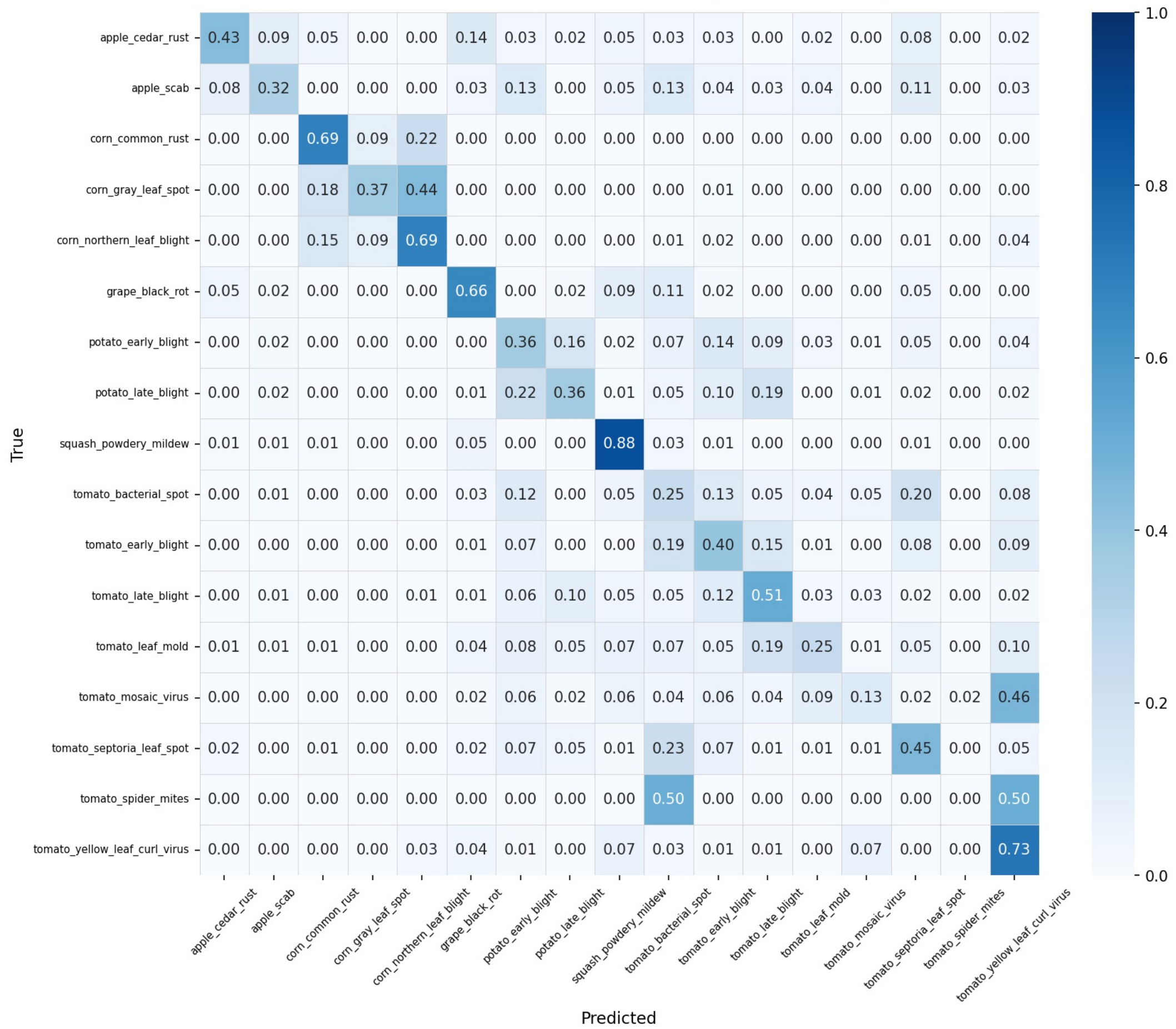
PlantDoc Eval — Confusion Matrix (row-normalised)
