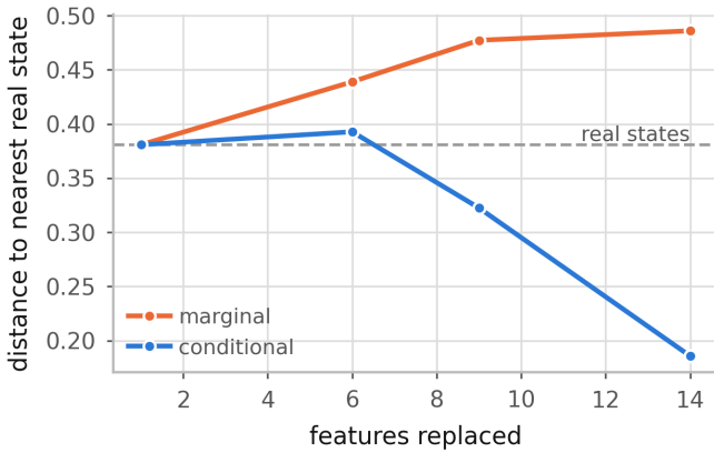
Figure 7: Distance from a masked state to the nearest real state, in per-feature standard deviations, against the number of features replaced. The dashed line is where real held-out states sit relative to the reference sample. Marginal masking moves above that floor as more features are replaced; neighbour-conditioned masking stays at or below it. The fully-masked point is omitted: those states are drawn from the reference sample itself, so their distance to it is zero by construction rather than by evidence.
