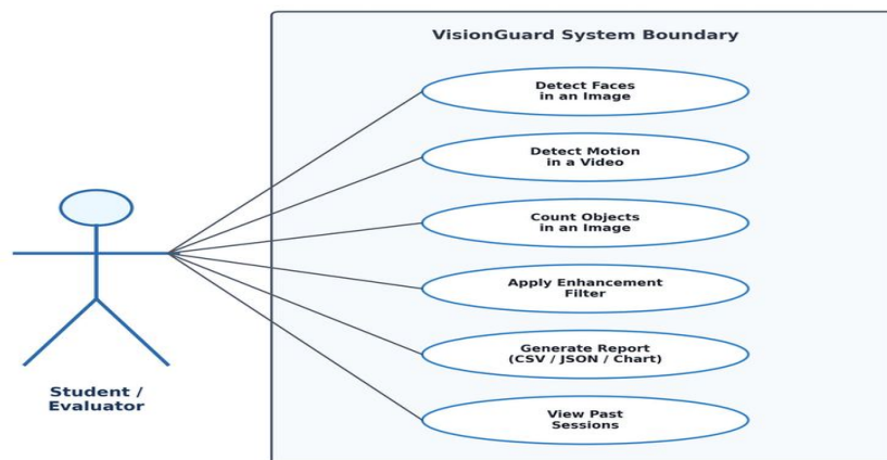
Figure 7.1 — Use Case Diagram
