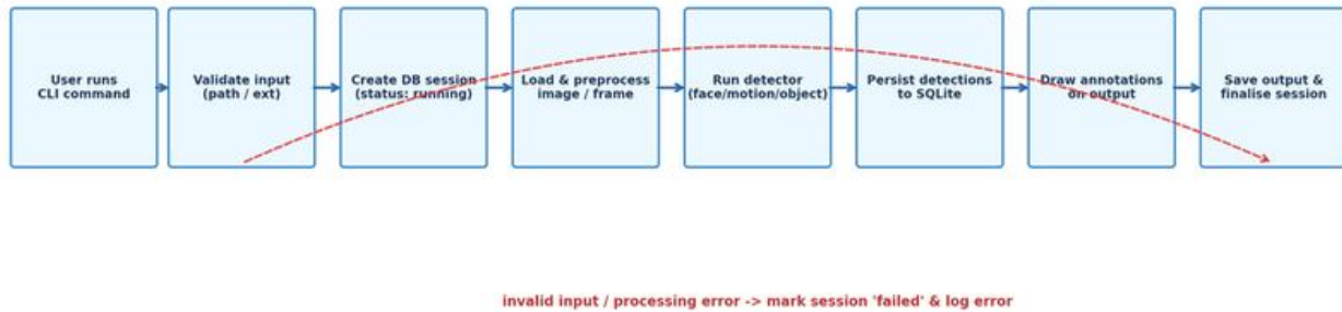
Figure 7.2 — Process Workflow Diagram
