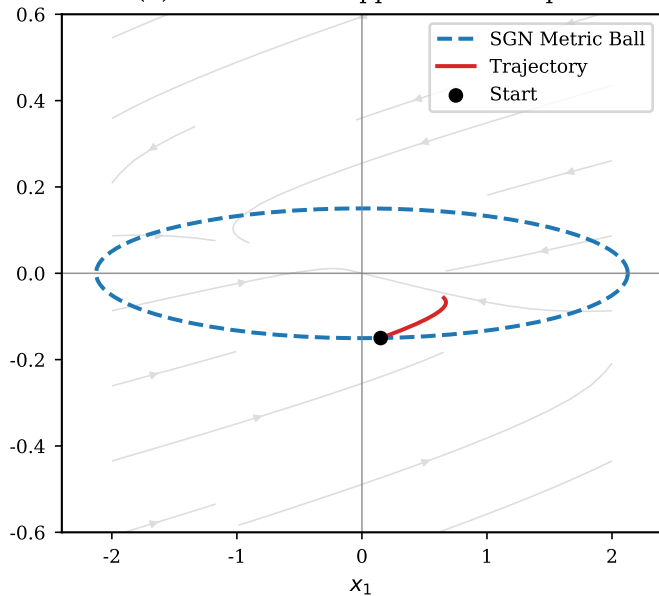
(b) SGN View: Trapped in the Ellipse
