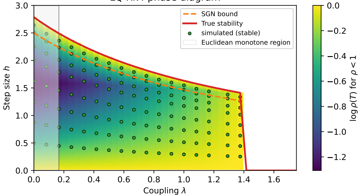
LQ Rk4 phase diagram
