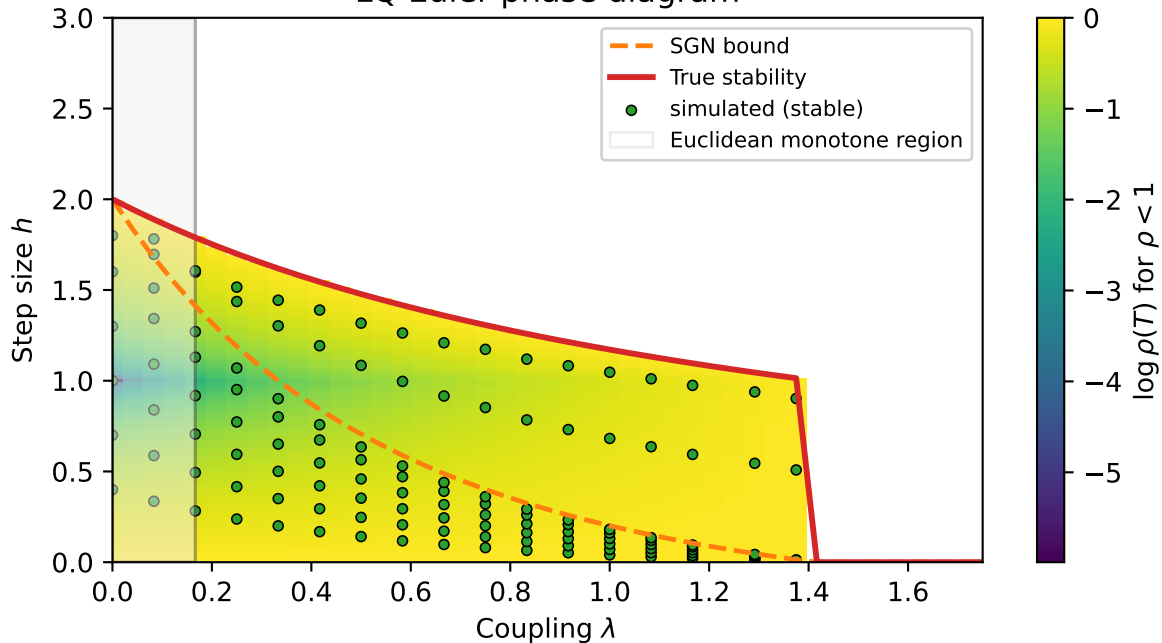
LQ Euler phase diagram
