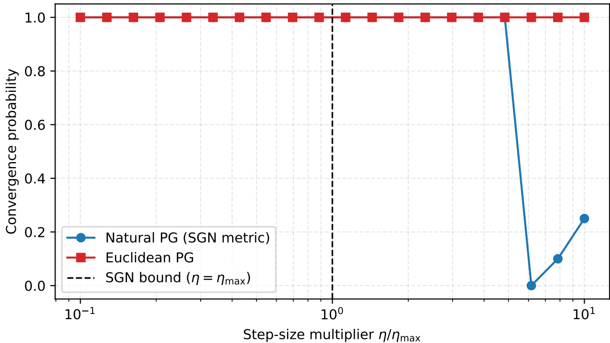
Markov game: stability vs step size
