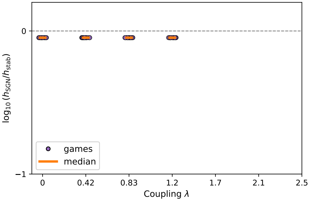
RK4 step bounds
