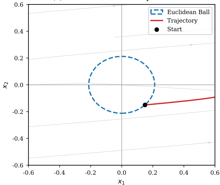
(a) Euclidean View: Escapes the Ball
