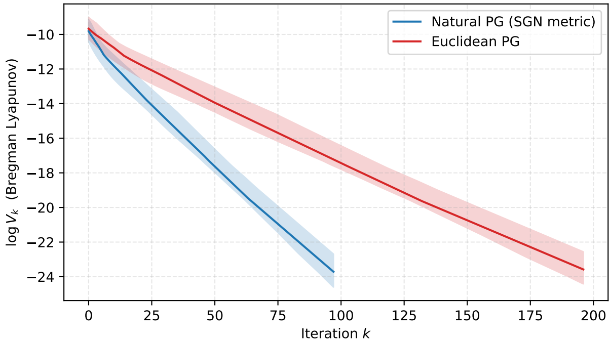
Markov game: Lyapunov decay in mirror geometry
