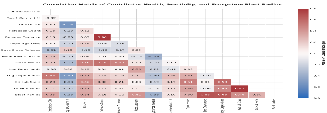
Figure 6: Pearson Correlation Heatmap across Contributor Concentration, Inactivity, Issue Triage, and Ecosystem Blast Radius.
