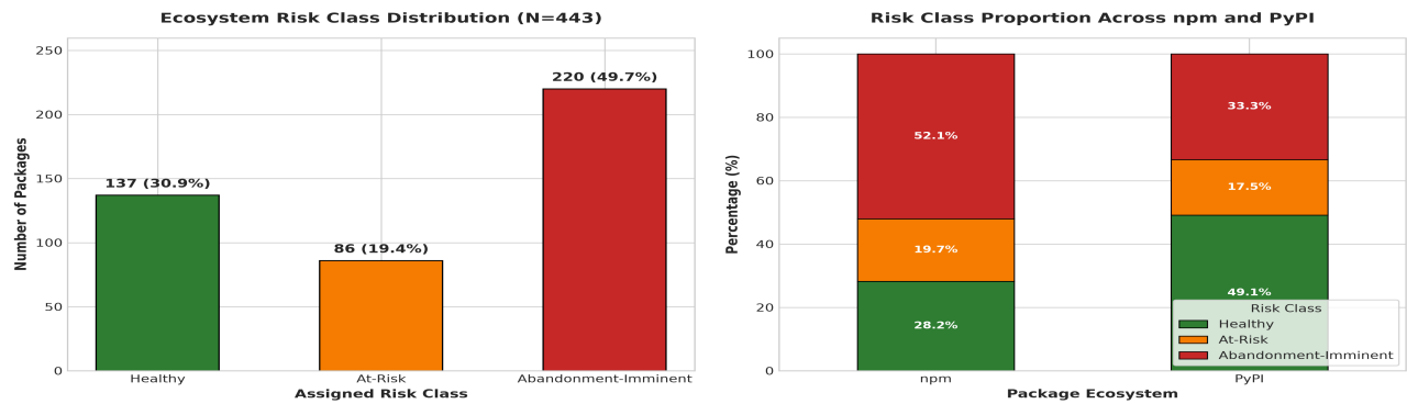
Figure 1: Ecosystem Risk Class Distribution overall (N=443) and cross-tabulated across npm and PyPI registries.
