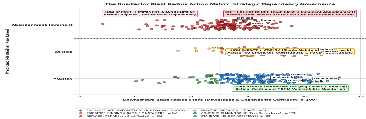
Figure 9: The Bus-Factor Blast Radius Strategic Action Matrix: Predicted Maintainer Risk vs Downstream Blast Radius. Action Matrix Interpretation: Packages clustering in the top-right quadrant (Quadrant 1) represent systemic, existential vulnerabilities—high blast radius combined with imminent abandonment. Quadrant 2 represents high-leverage intervention targets where corporate sponsorship can expand maintainer redundancy before burnout triggers abandonment.
