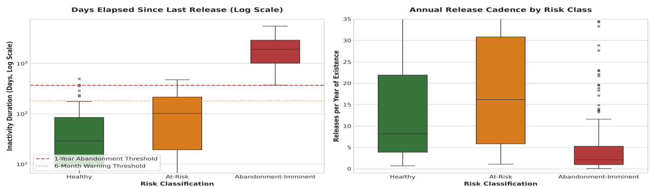
Figure 2: Maintenance Inactivity duration (days elapsed since last release, log scale) and Annualized Release Cadence across Risk Classes.
