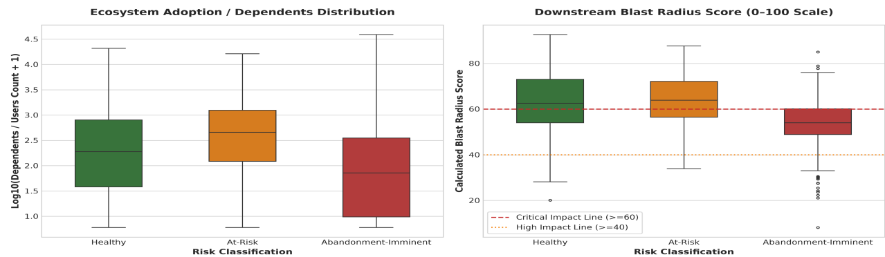
Figure 5: Downstream Dependents and Calculated Blast Radius Index (0–100 Scale) across Risk Classes.
