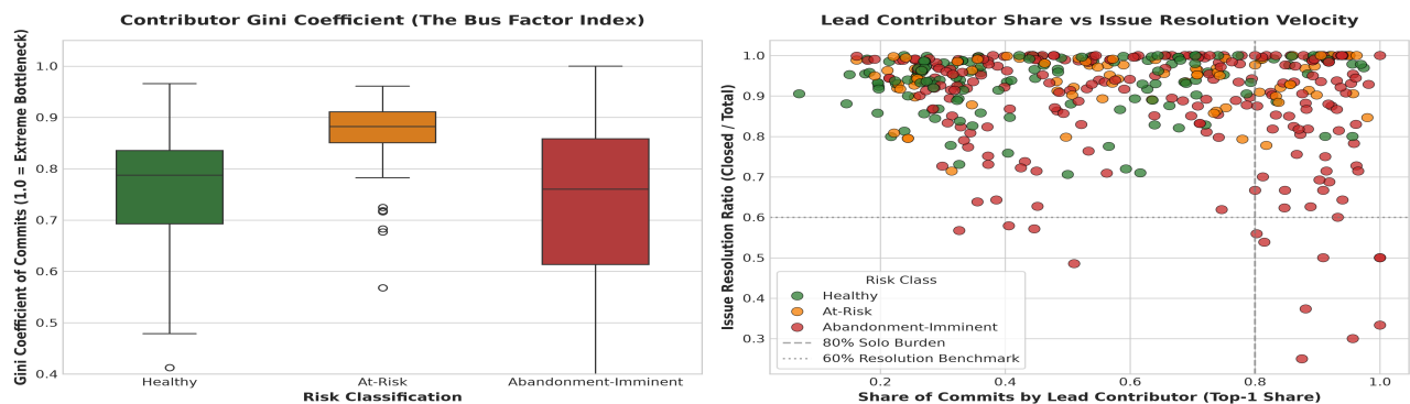
Figure 3: Contributor Gini Coefficient (The Bus Factor Index) and Lead Contributor Commit Share vs Issue Resolution Velocity.
