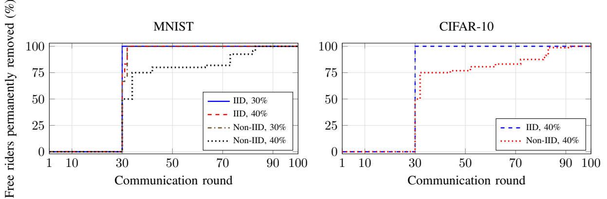
Fig. 1. Cumulative permanent removal of free riders by communication round. Curves use the same best-observed per-attack selections as Table I; the vertical guide marks round 30, the earliest statistical-removal point under the configured schedule.
