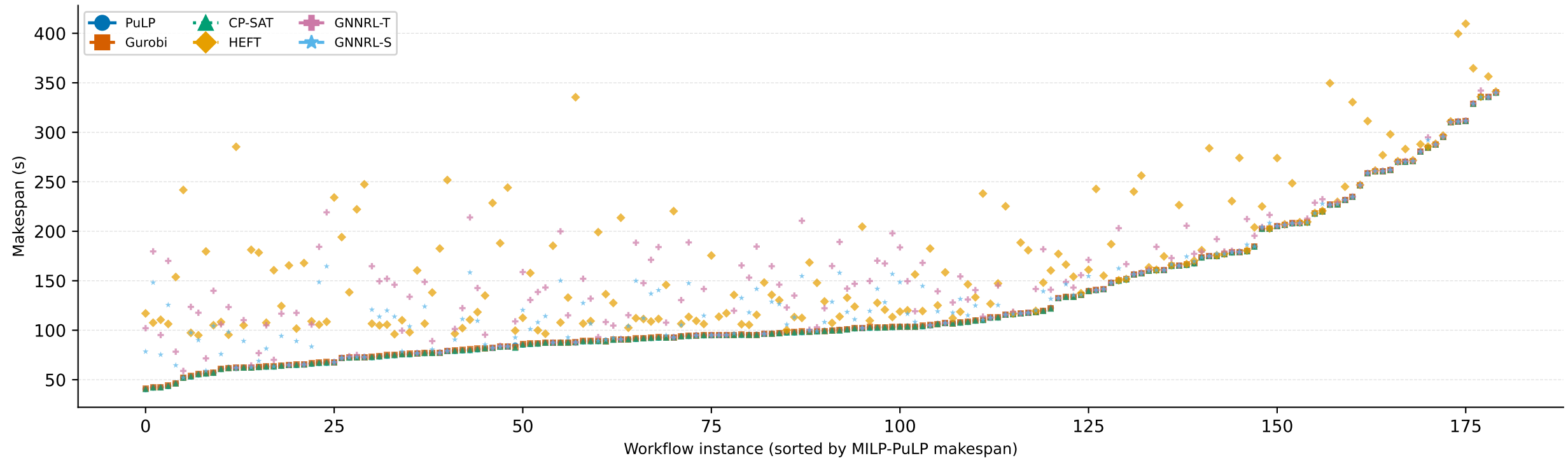
Per-Instance Makespan | RNC100 Hetero mode
