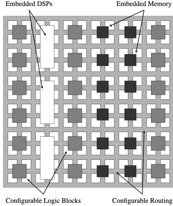
Figure 2.11: General layout of an FPGA. CLBs, DSPs, and memory blocks are placed in a configurable routing network.
