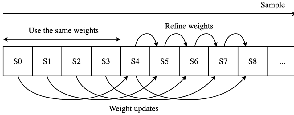
Figure 3.2: The proposed weight update scheme by Jia et al. Weights are kept unchanged for the first samples of every line, after which the sample from four samples earlier is used in the weight update calculation.
