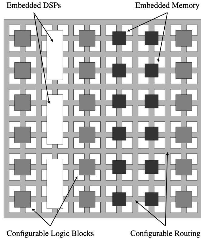
Figure 2.9: General layout of an FPGA. CLBs, DSPs, and memory blocks are placed in a configurable routing network.
