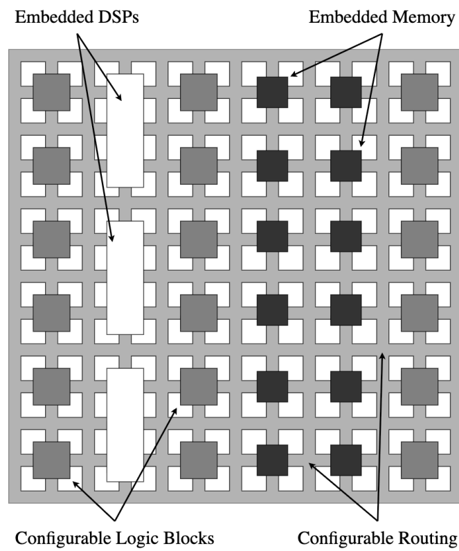
Figure 2.9: General layout of an FPGA. CLBs, DSPs, and memory blocks are placed in a configurable routing network.
