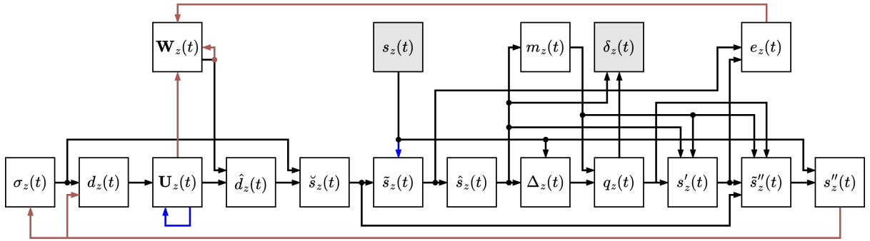
Figure 2.9: Data dependencies of the issue 2 predictor with t - 1 and z - 1 dependencies marked in red and blue respectively.
