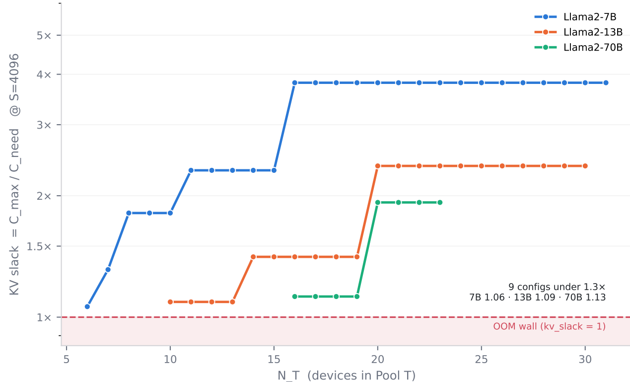
Pool T capacity gate: every in-flight request holds KV on every block
