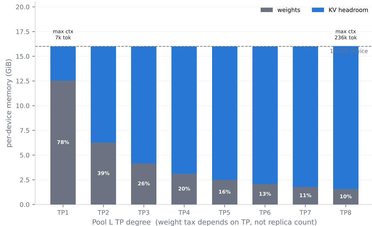
Llama2-7B: a low-TP replica spends the device on weights
