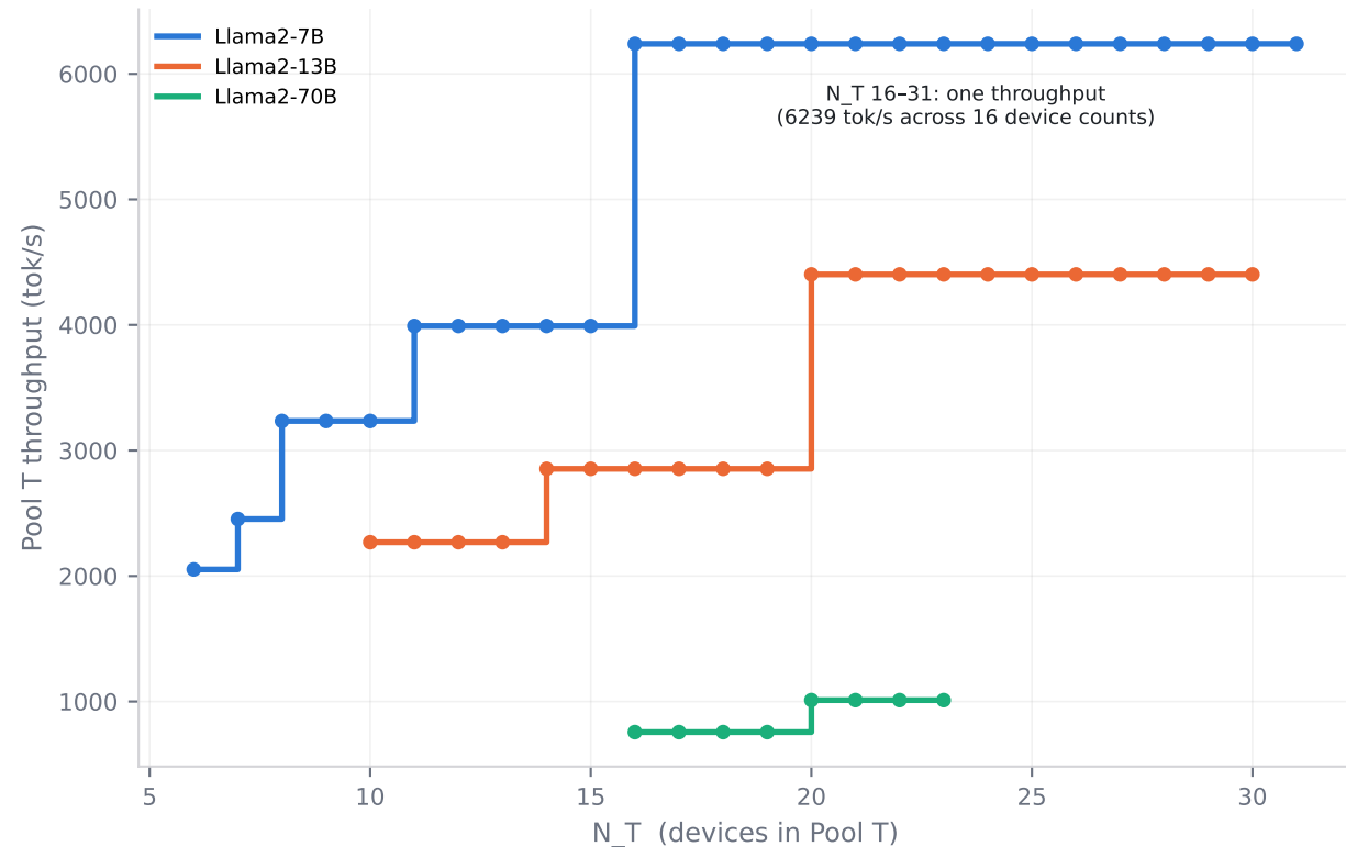
Throughput: a staircase — flat inside a tier
