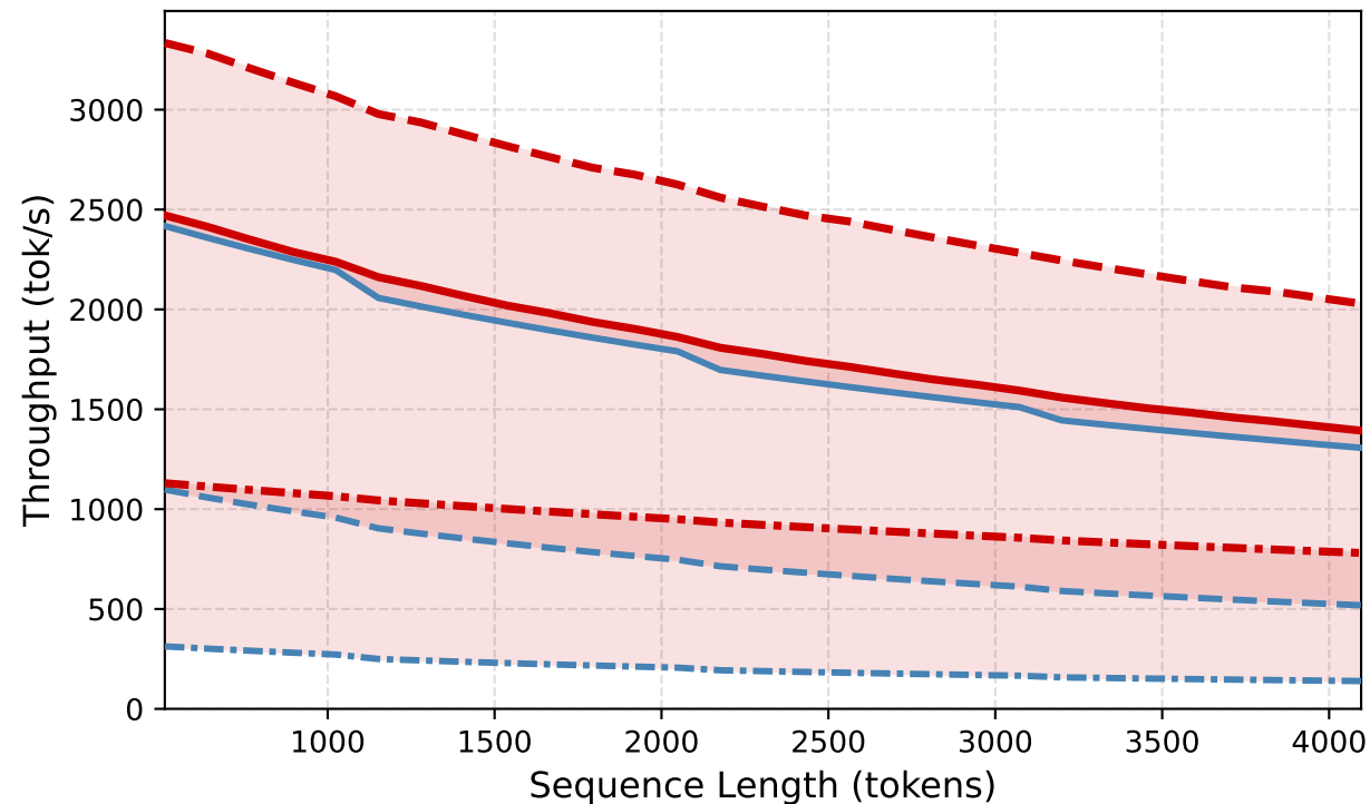
(b) Throughput vs Seqlen — Long Requests (seqlen > 512) Shaded = Pool T throughput gain over balanced static 7B: ~1× (negligible), 13B: ~3×, 70B: ~4×
