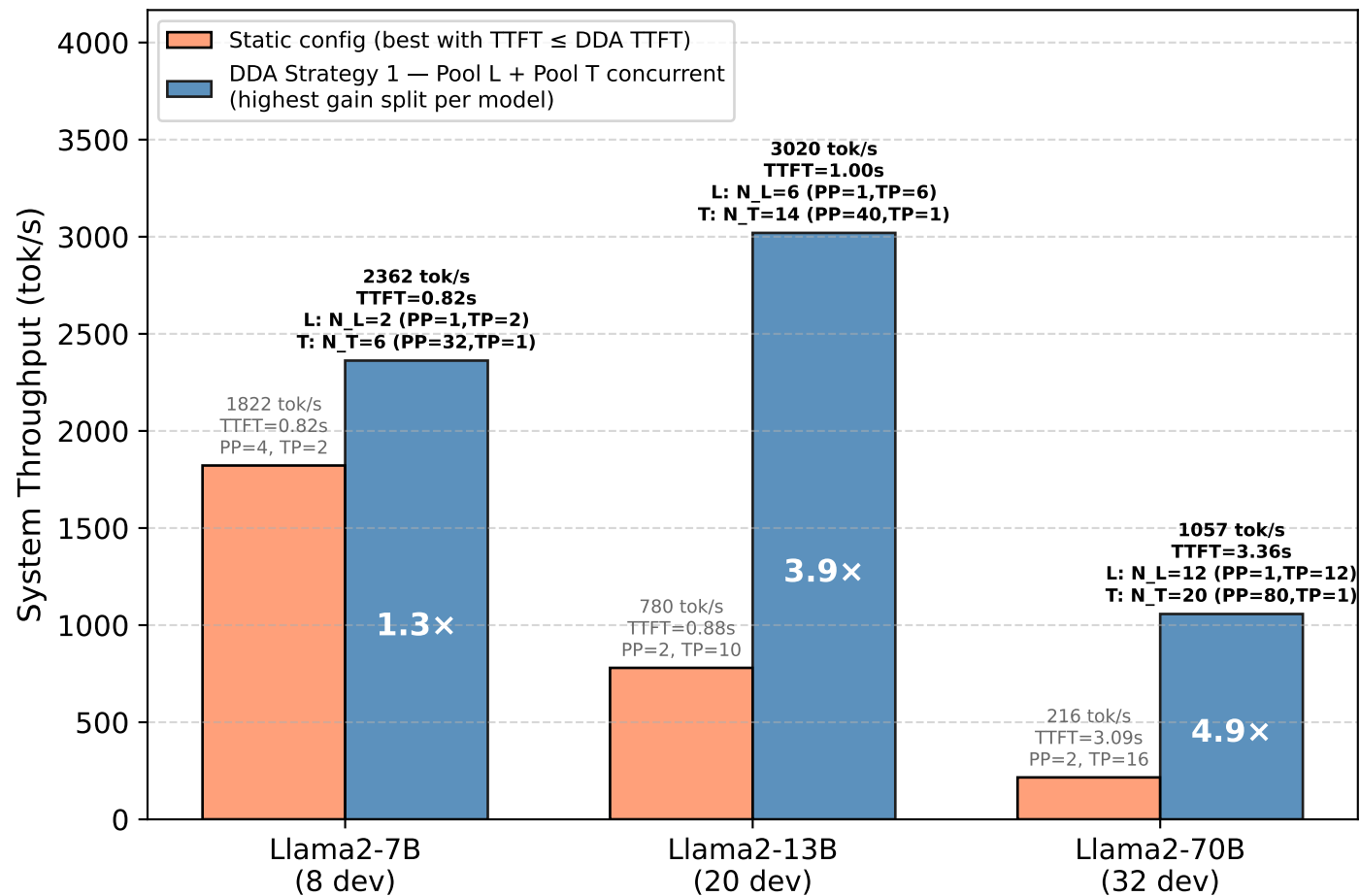
(b) Best-Gain DDA Split vs Static — Same TTFT Constraint
