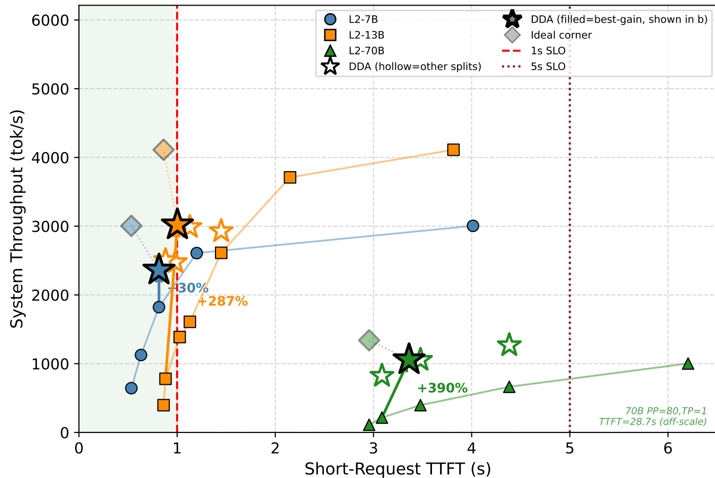
(a) DDA vs Static Pareto — Zoomed [0–6s]
