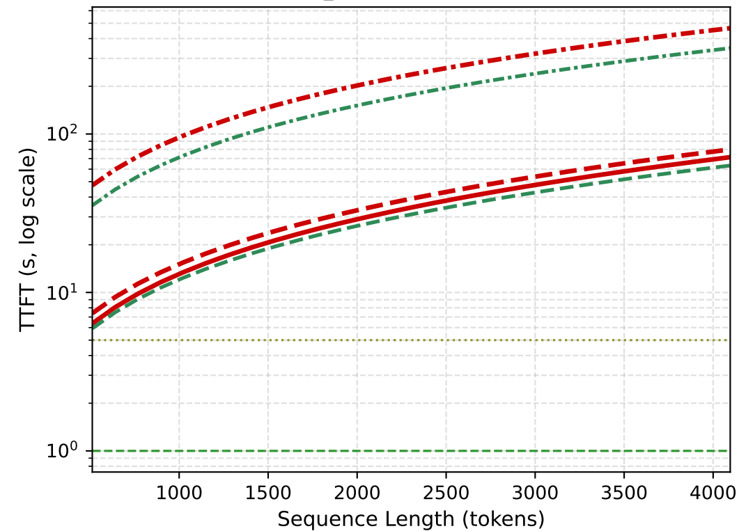
(c) Long-Seq Pool T TTFT S2 N_T = optimal at \alpha=0.35
