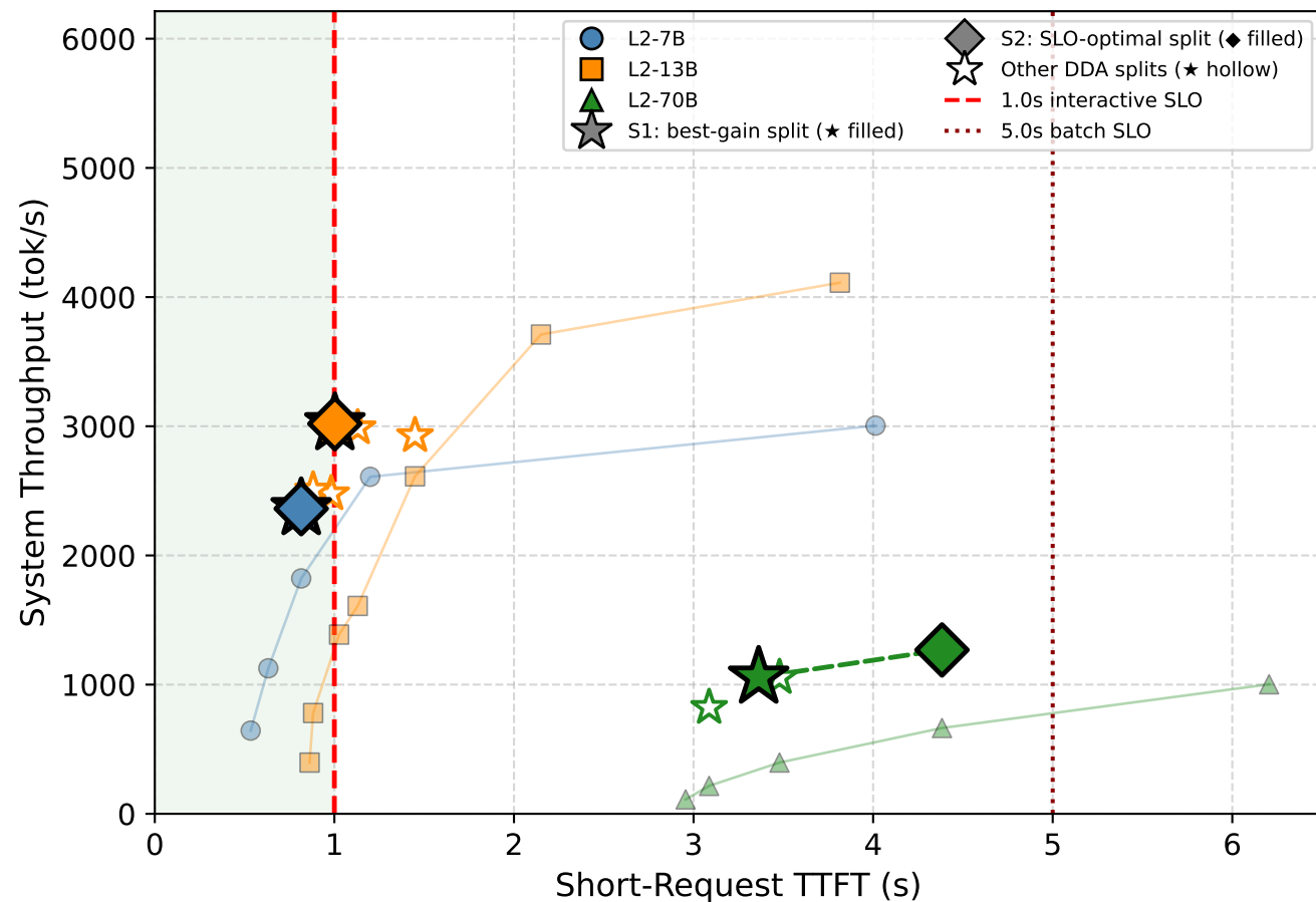
(a) S1 vs S2 — Pareto Scatter [0-6s]
