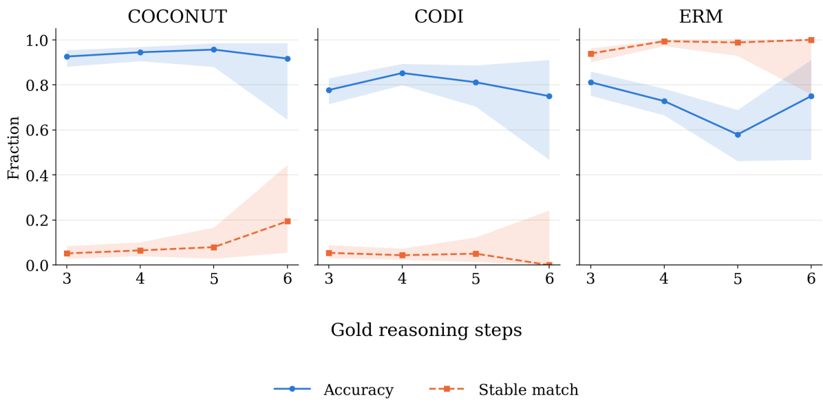
Figure 7: Testing accuracy and stable match score with increasing gold reasoning steps (ProsQA). As Figure 3, but bucketed by the length of each sample’s gold reasoning chain instead of calculator-notation steps. Shaded region is a 95% confidence interval: a Wilson score interval for accuracy, and a BCa bootstrap confidence interval (10,000 resamples) over per-question stable match fractions for stable match. Accuracy is roughly flat across buckets for all three models, and COCONUT and CODI’s stable match remains near zero throughout, in contrast to the GSM8k trend in Figure 3.
