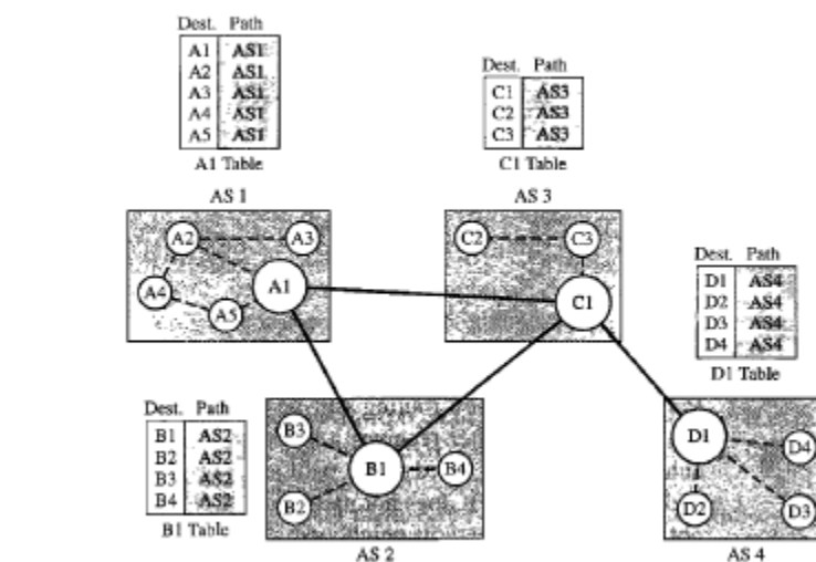
Figure 22.30 Initial routing tables in path vector routing
