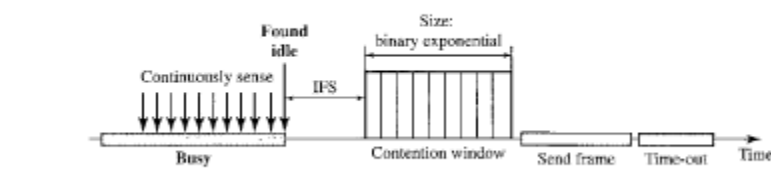
Figure 12.16 Timing in CSMA/CA
