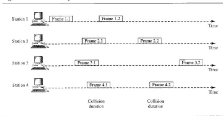
Figure 12.3 Frames in a pure ALOHA network
