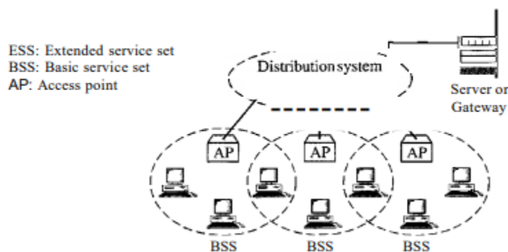
Extended service sets (ESSs)
