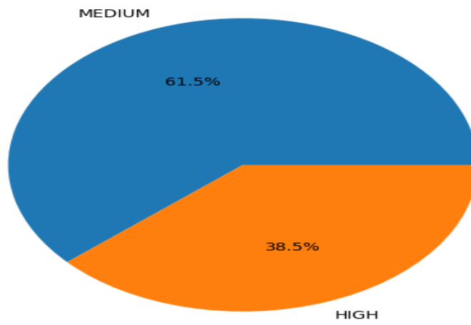
Severity Distribution
