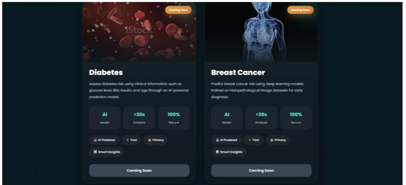
Fig 6: Disease Predictors
