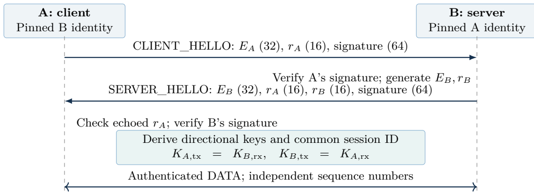
Figure 3: Two-message setup. Field lengths are bytes and exclude the 28-byte common header. E_A, E_B are ephemeral public keys; r_A, r_B are random values.
