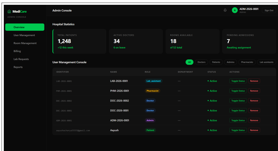
Figure 4.4: Admin dashboard
