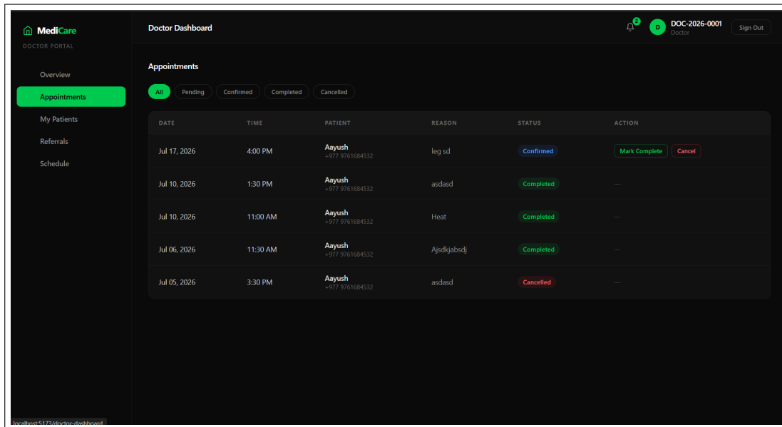
Figure 4.3: Doctor dashboard
