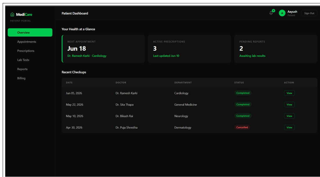
Figure 4.2: Patient dashboard
