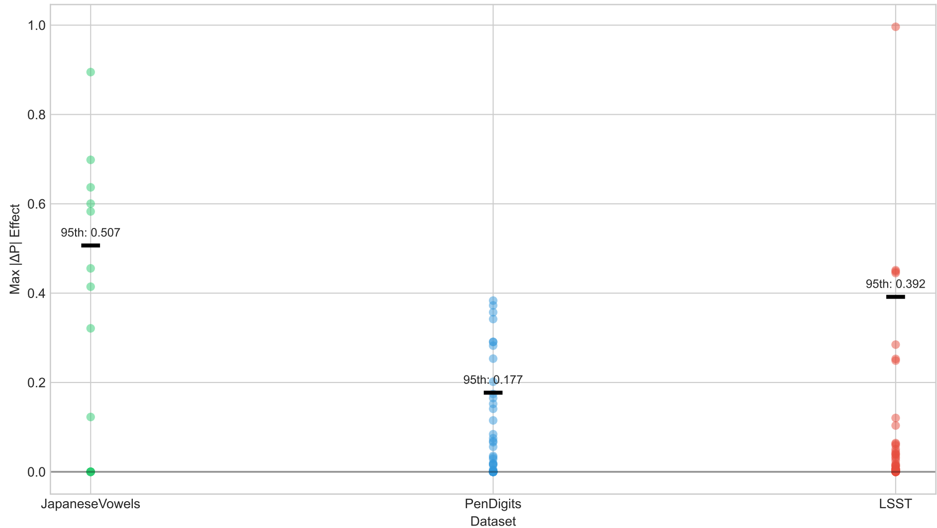
Observed Effects vs Null Distribution 95th Percentile
