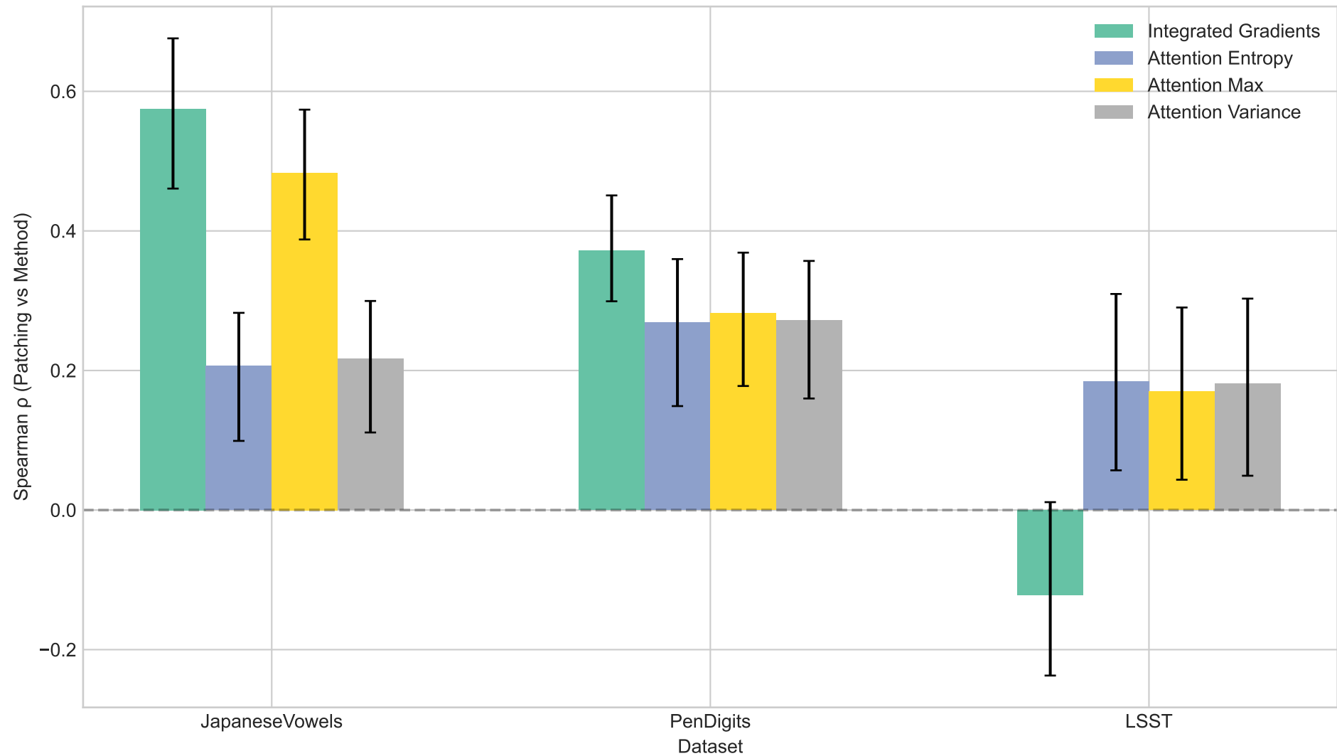
Activation Patching vs Alternative Methods
