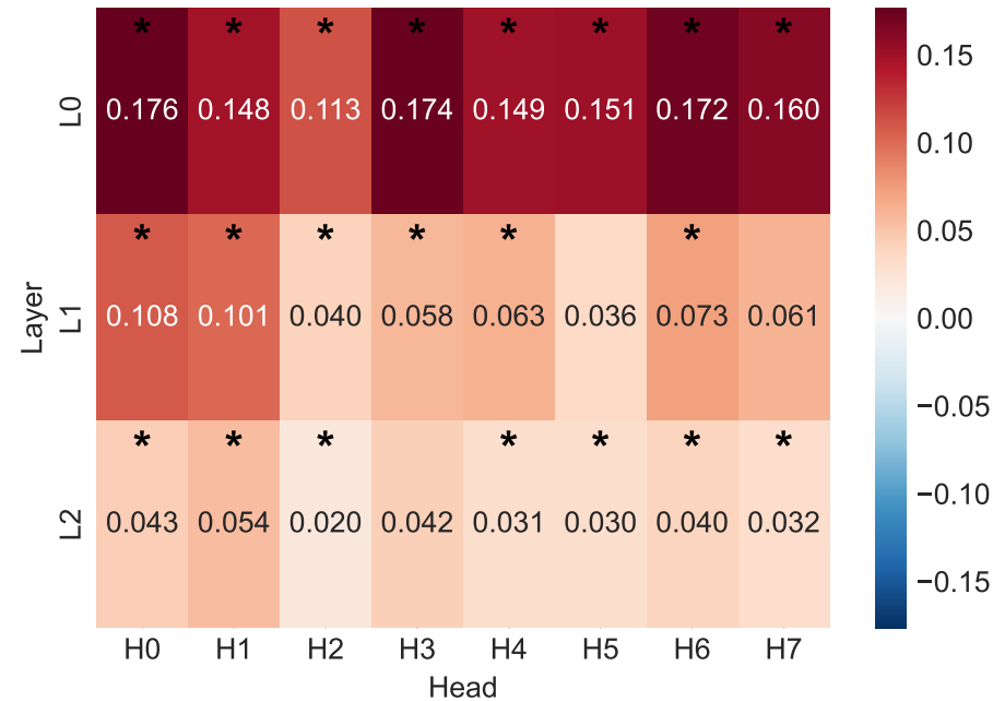
JapaneseVowels (* = FDR p < 0.05 )
