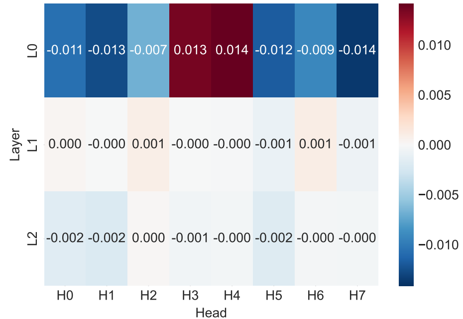
LSST (* = FDR p < 0.05 )
