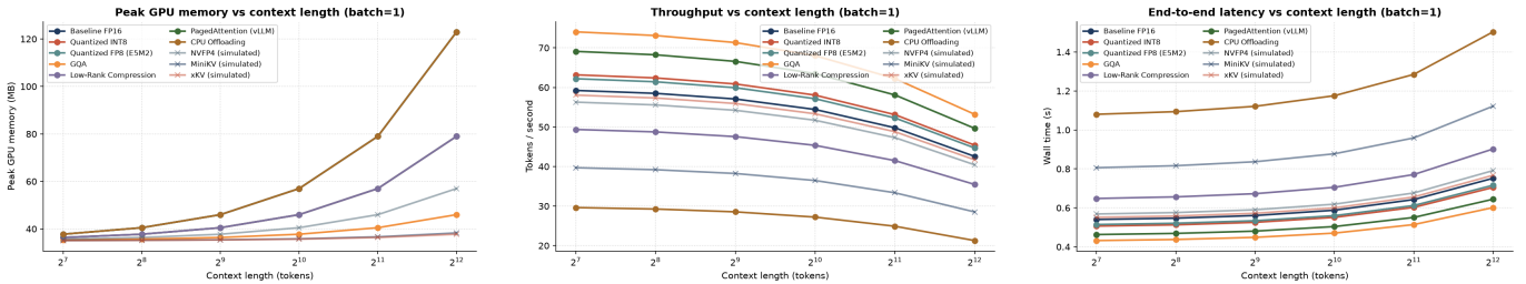
Fig. 2. Behaviour of the simulated techniques as the context length grows at batch=1. Left: peak GPU memory versus context length; the GQA curve is the lowest among the architectural techniques, while MiniKV and xKV reach the lowest absolute cache sizes. Centre: throughput in tokens per second; quantization preserves the FP16 throughput baseline while compression and eviction add small overheads. Right: per-token latency on a log scale; PagedAttention and the baseline dominate the low-latency region, while CPU Offloading pays a fixed transfer cost per generated token.
